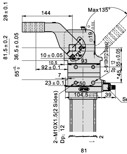
Horizontal clamping position
