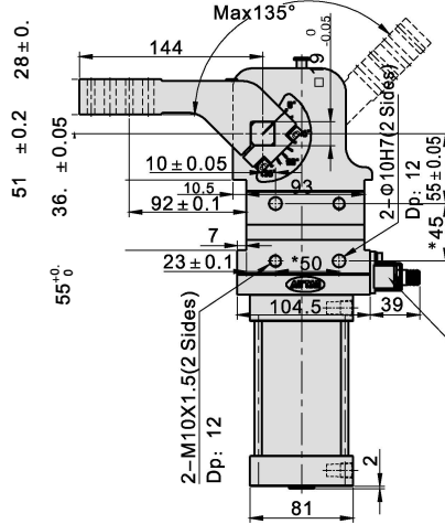
Horizontal clamping position
