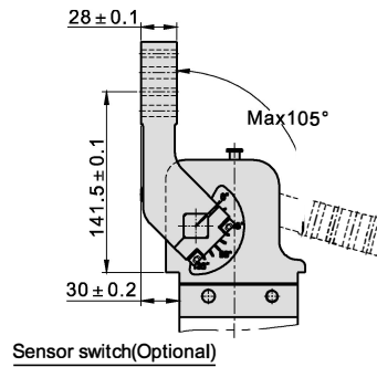
Vertical clamping position
